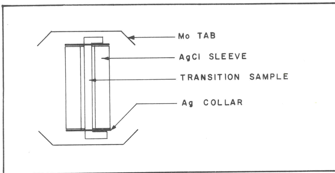
Figure 25.-Pressure Calibration Assembly.
